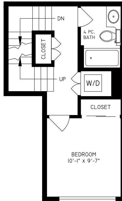
SECOND FLOOR 337 SQ. FT. 8'-0" CEILING HEIGHT
